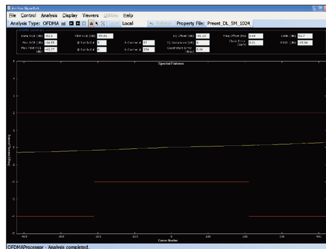
Figure 6. In a spectral flatness measurement, the power of the spectral lines is compared to a reference, such as the total transmitted power in a burst, to determine transmitter compliance to the WiMAX standard.
